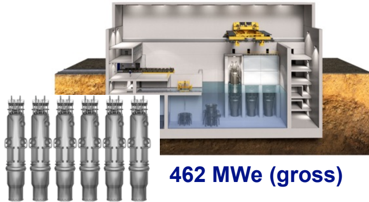
6-module plant
