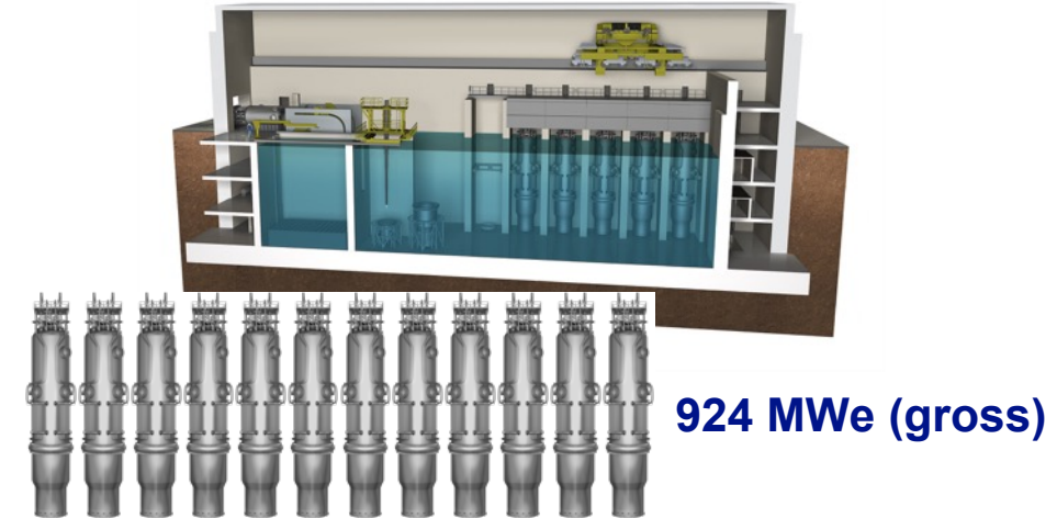
12-module plant
